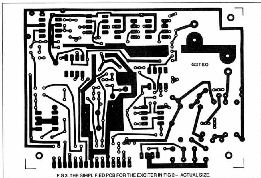
FIG 3. THE SIMPLIFIED PCB FOR THE EXCITER IN FIG 2 - ACTUAL SIZE.
