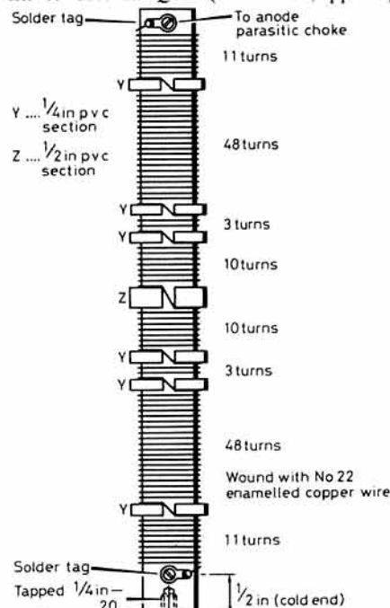
FIG 4. AA6GK's ANODE-CIRCUIT OF RF CHOKE FOR HIGH-POWER AMPLIFIERS AVOIDS RESONANCES ON MOST HF BANDS. BUT ALL SUCH CHOKES SHOULD PREFERABLY BE CHECKED IN SITU SINCE NEARBY METALWORK WILL SHIFT THE RESONANCE FREQUENCIES.
