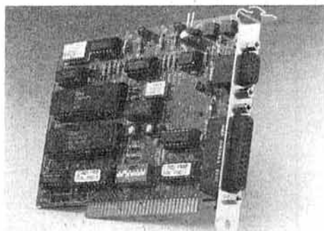
PC * PACKET ADAPTER
