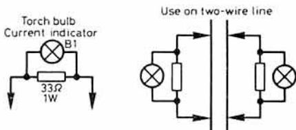
FIG 6. USING INEXPENSIVE PILO-LAMP BULBS AS RF CURRENT INDICATORS. CLIP ACROSS A FEW INCHES OF ANTENNA FEED-WIRE. VARY RESISTOR VALUE TO MATCH LINE CIRCUIT ETC.
