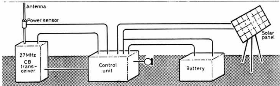
FIG 1. A VILLAGE TERMINAL IN THE SIERRA LEONE LOW-COST RURAL TELECOMMUNICATIONS PROJECT BEING IMPLEMENTED WITH THE ASSISTANCE OF DR S A G CHANDLER, G3UDD/9L1SC OF THE UNIVERSITY OF WARWICK.
